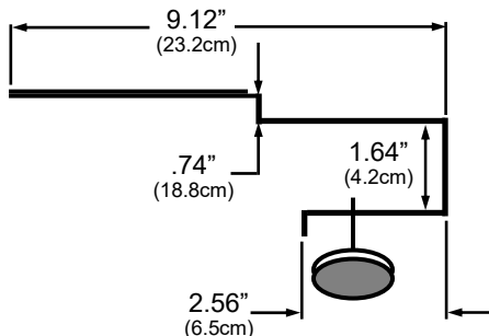
Pocket Attachment
