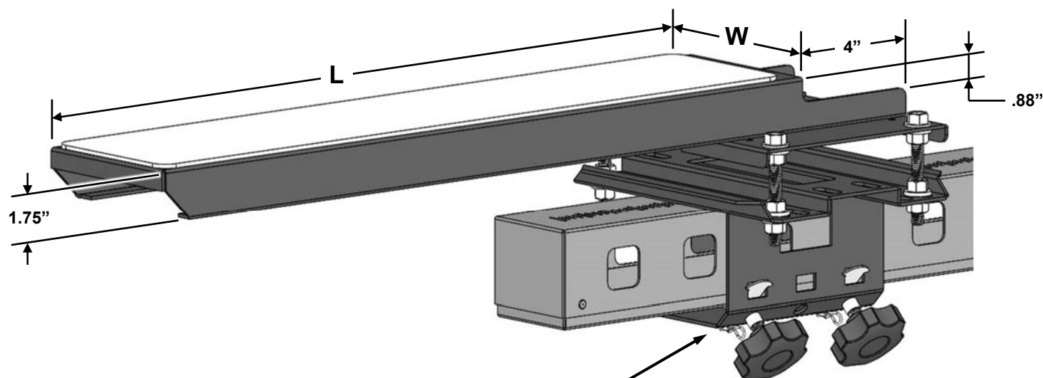
Pallet Arm V-2000 P/N: V2-ARM (shown) V-1000 P/N: V1-ARM
